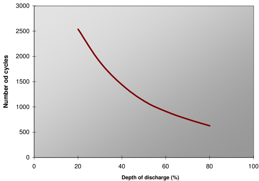
Number of cycles versus depth of discharge
