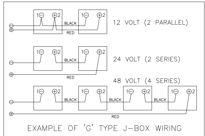
Figure 3. Standard Wiring Examples
