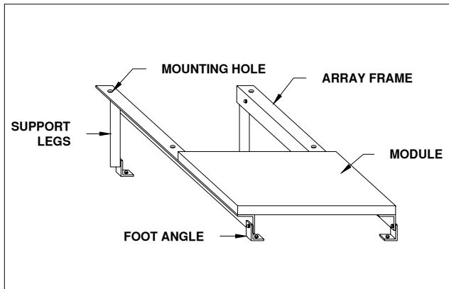
Figure 2. Basic Rack or Standoff Mounting Structure
