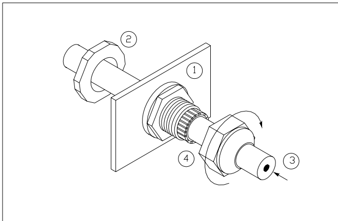
Figure 5. Installation Example of Cable Clamp
